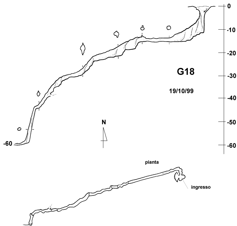
Fig. 5 – Profile and plan view of an inclined moulin (G18: survey Ass. La Venta, October 1999)
